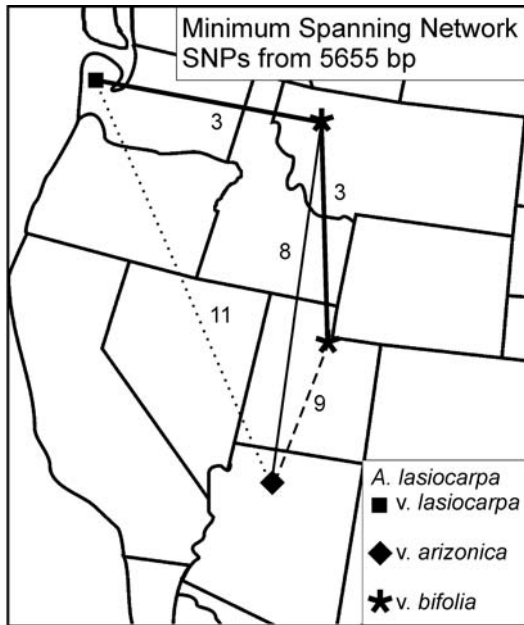
Figure 6. Minimum spanning network based on 5655 bp of sequence data. The numbers next to the links are the number of SNPs (including indel information).
